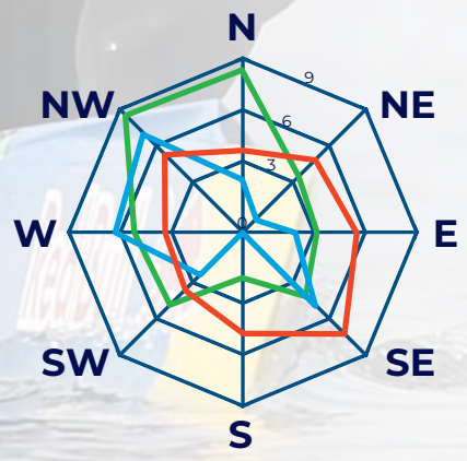
Relative frequencies of wind's direction in dependence of average velocity for the period of May 1. – 15. 2014 – 2019
